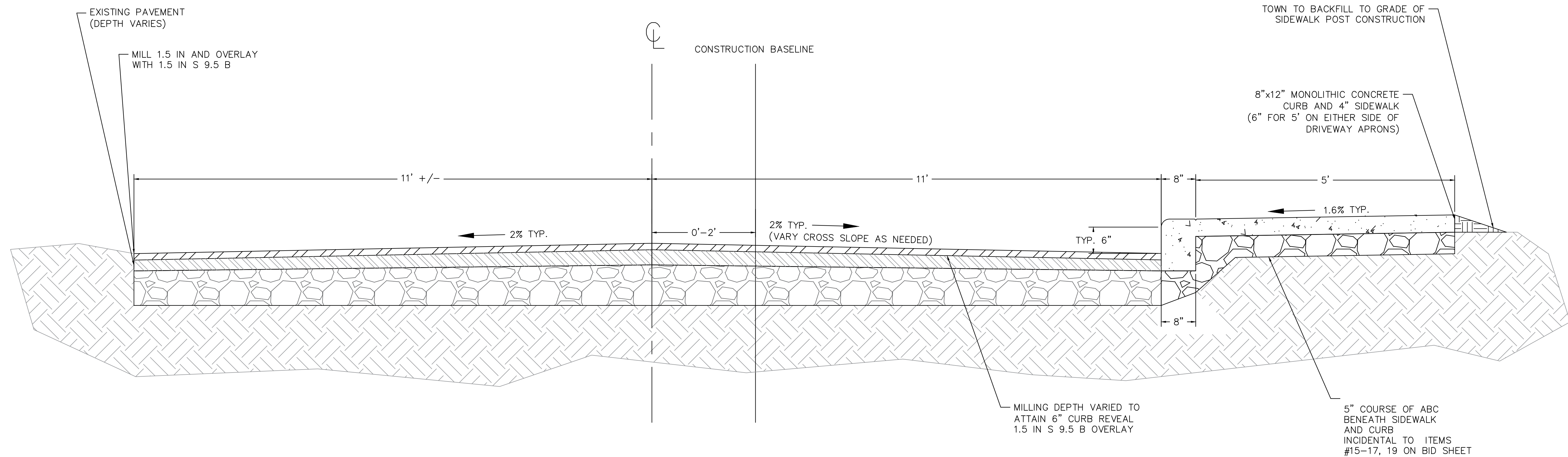
TYPICAL STREET AND SIDEWALK SECTION: MAPLE TO SWEET BAY NOT TO SCALE
