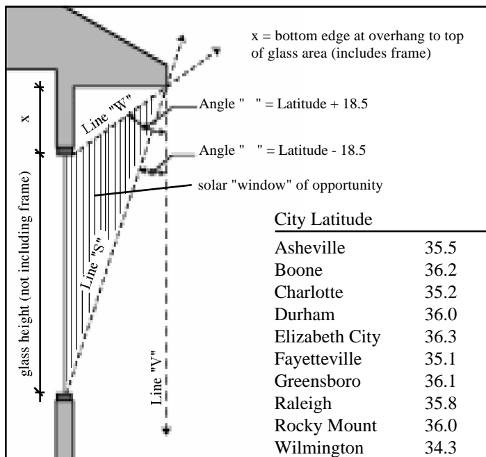
Figure 2. Diagram for sizing overhang
