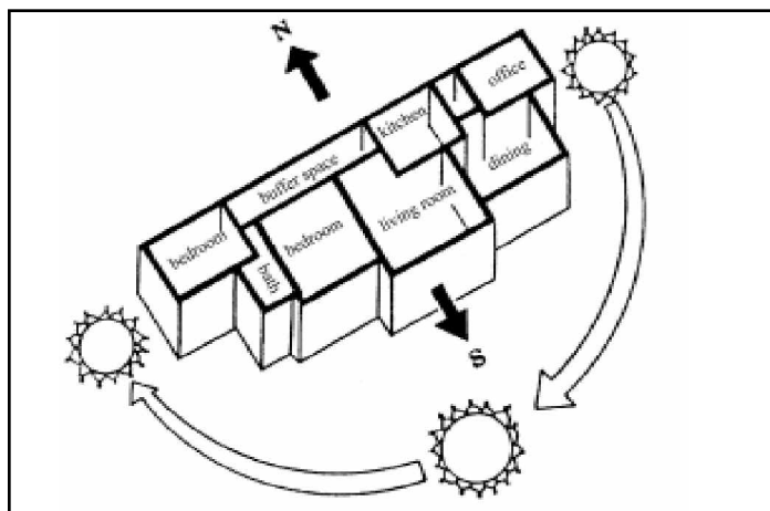
Figure 3. Place rooms where they are compatible with the sun's path. Buffer spaces should be placed to the north.
